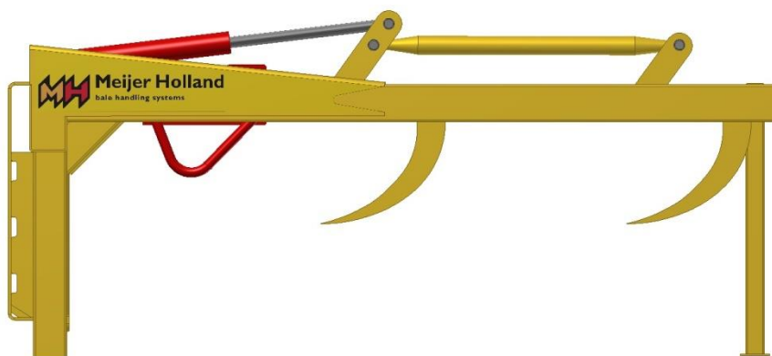
Movement hooks
